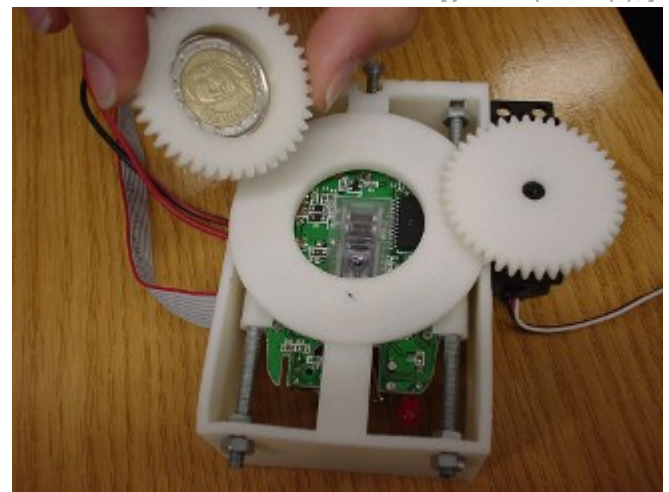
/export/sites/universitat-lleida/ca/serveis/oficina/Noticies/17-de-novembre-2009 Prototype used in the detection tests
